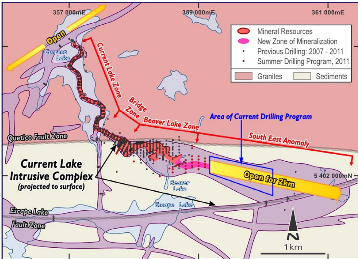
Figure 3. The Current Lake Intrusive Complex showing the area of the current step-out drilling program (refer to Magma announcement dated September 29, 2011).
