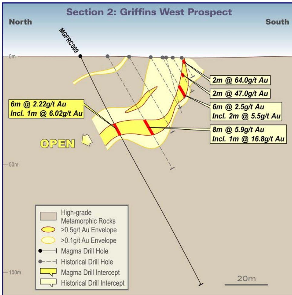
Figure 3. Griffins West Prospect Cross-Section 622420E.
