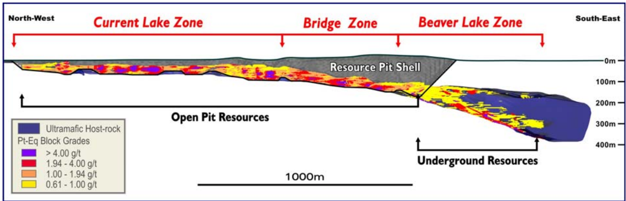
Figure 1. Long section showing resource model and optimized open pit shell.
