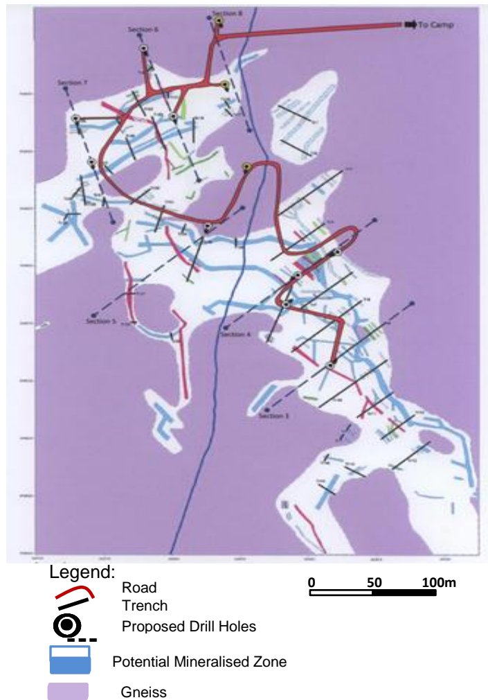
Figure 2: Geological map showing potential drill target areas identified from mapping – note location of the Tembo drill target in the east of Wigu Hill
