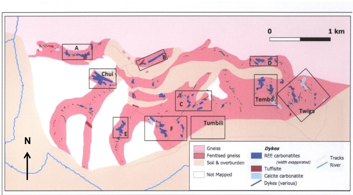
Figure 2: Geological map showing potential drill target areas identified from mapping – note location of the Tembo drill target in the east of Wigu Hill
