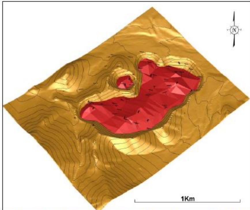
Figure 1: Chita Conceptual Pit Constrained Inferred Resource Diagram (oblique view looking North).
