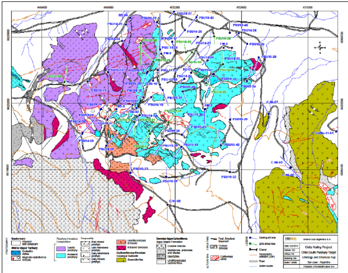
Map 1: Chita Porphyry Surface Geology and Drill Hole Locations
