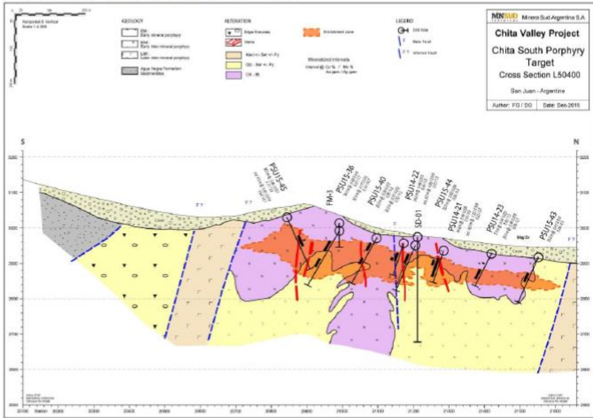
Map 3: Chita Porphyry Typical Cross Section
