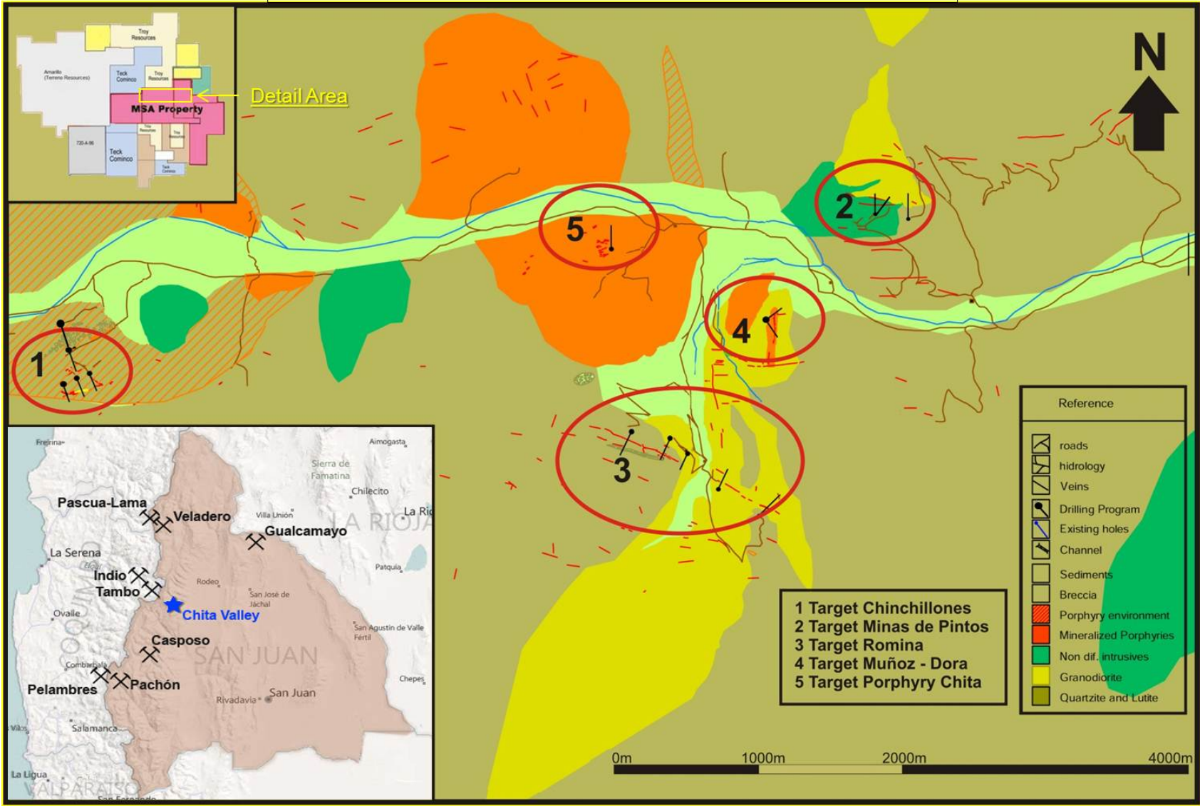
Figure 1: Chita Valley Property, geology, location of target areas for Phase I diamond drilling.
