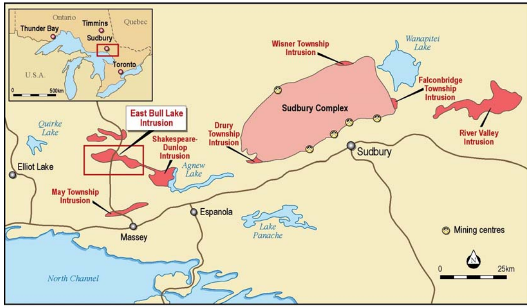
Figure 1: Location of East Bull Lake intrusion
