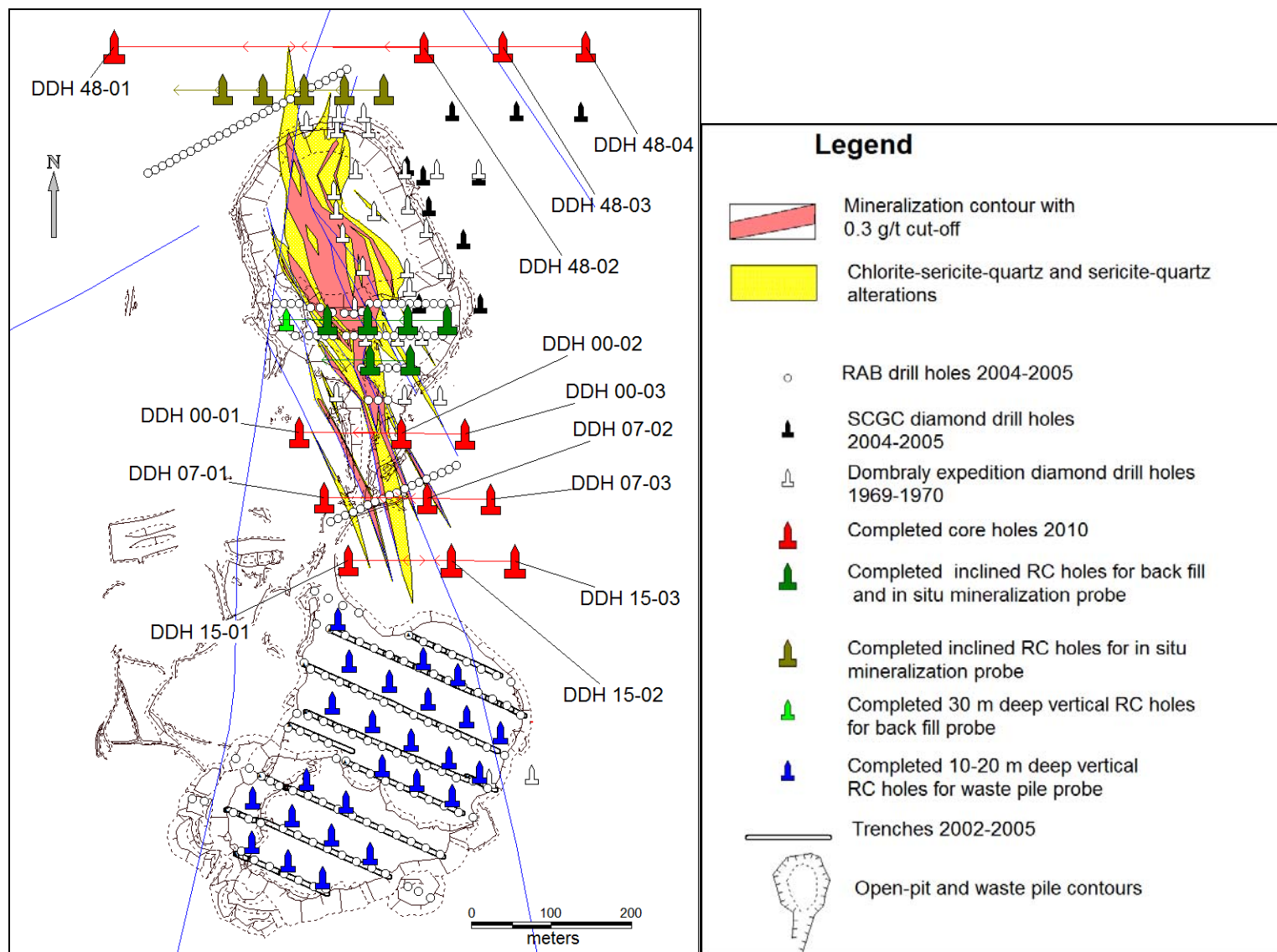
Figure 3 – Dombraly Core and RC Drilling Locations
