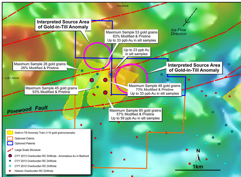
Figure 2. Conqueror Anomaly drillhole plan and interpretation on total magnetic intensity (TMI) image showing extent of gold-in-till anomaly and recent silt and bedrock gold results.
