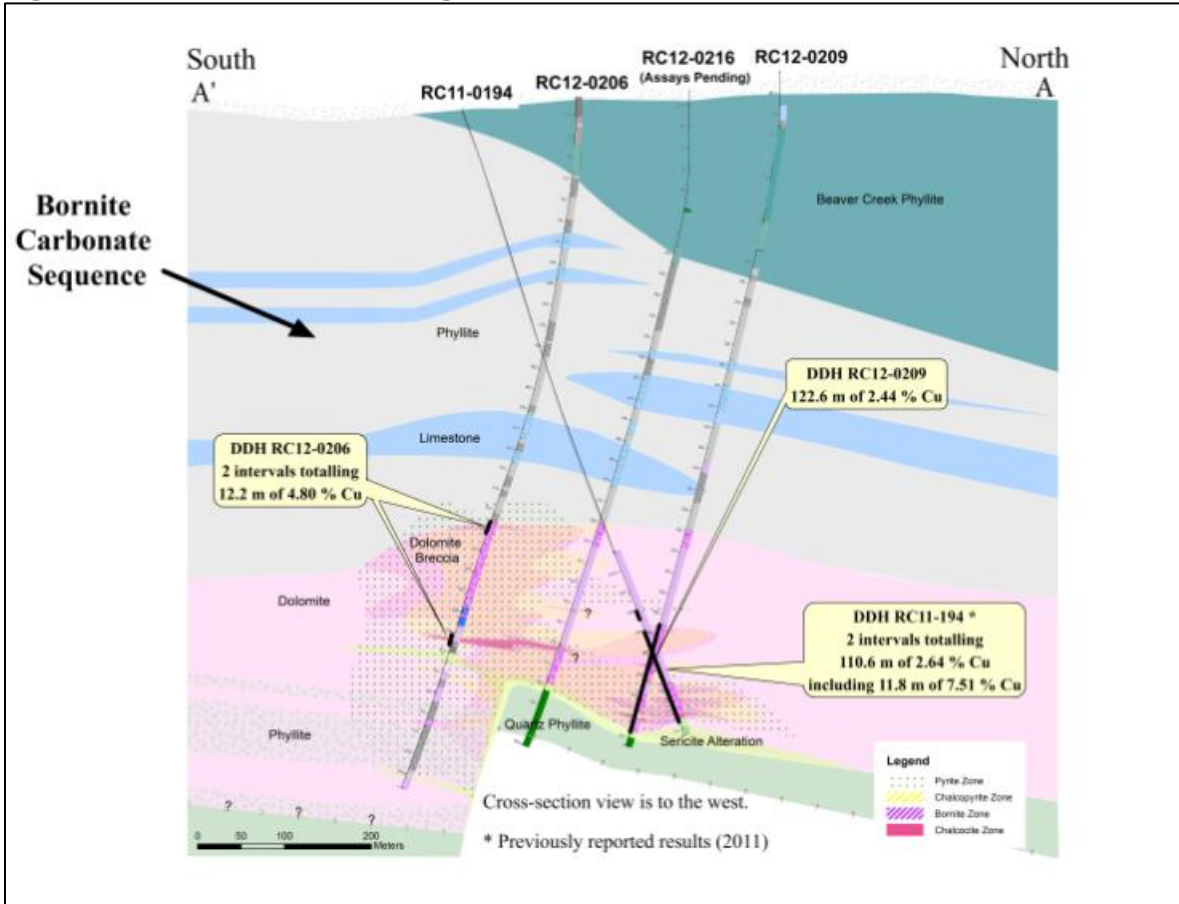
Figure 2: Cross-section through the South Reef Zone
