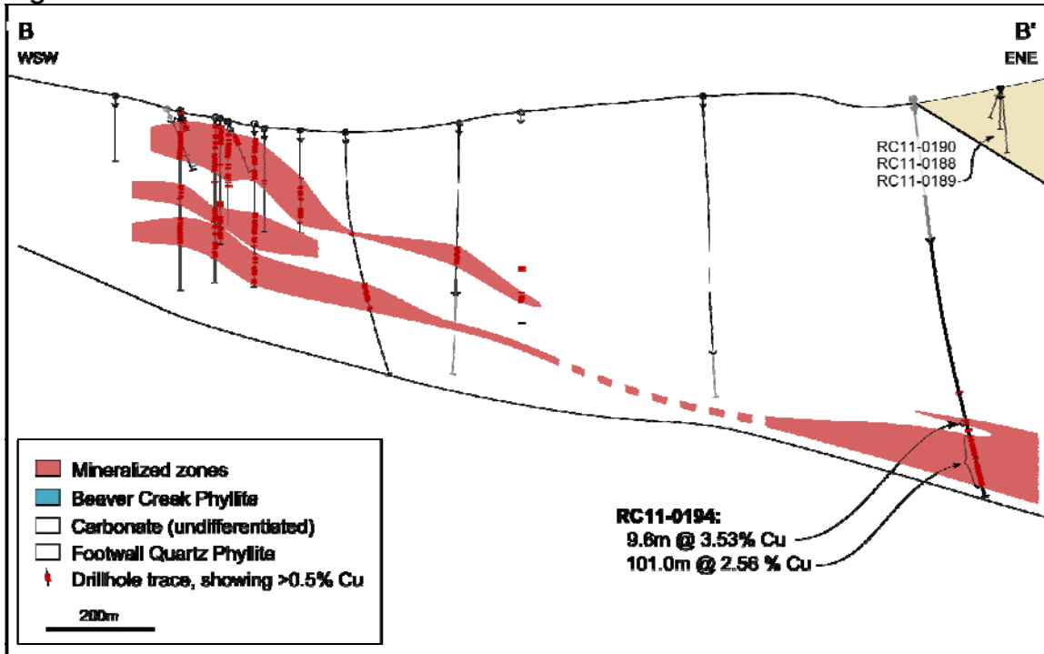
Figure 3: Bornite Cross Section B-B'
