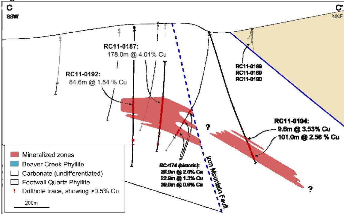
Figure 4: Bornite Cross Section C-C'
