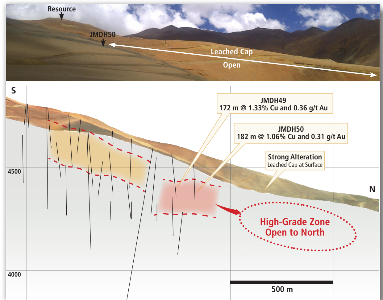
Josemaria Project, Argentina North-South Vertical Section
