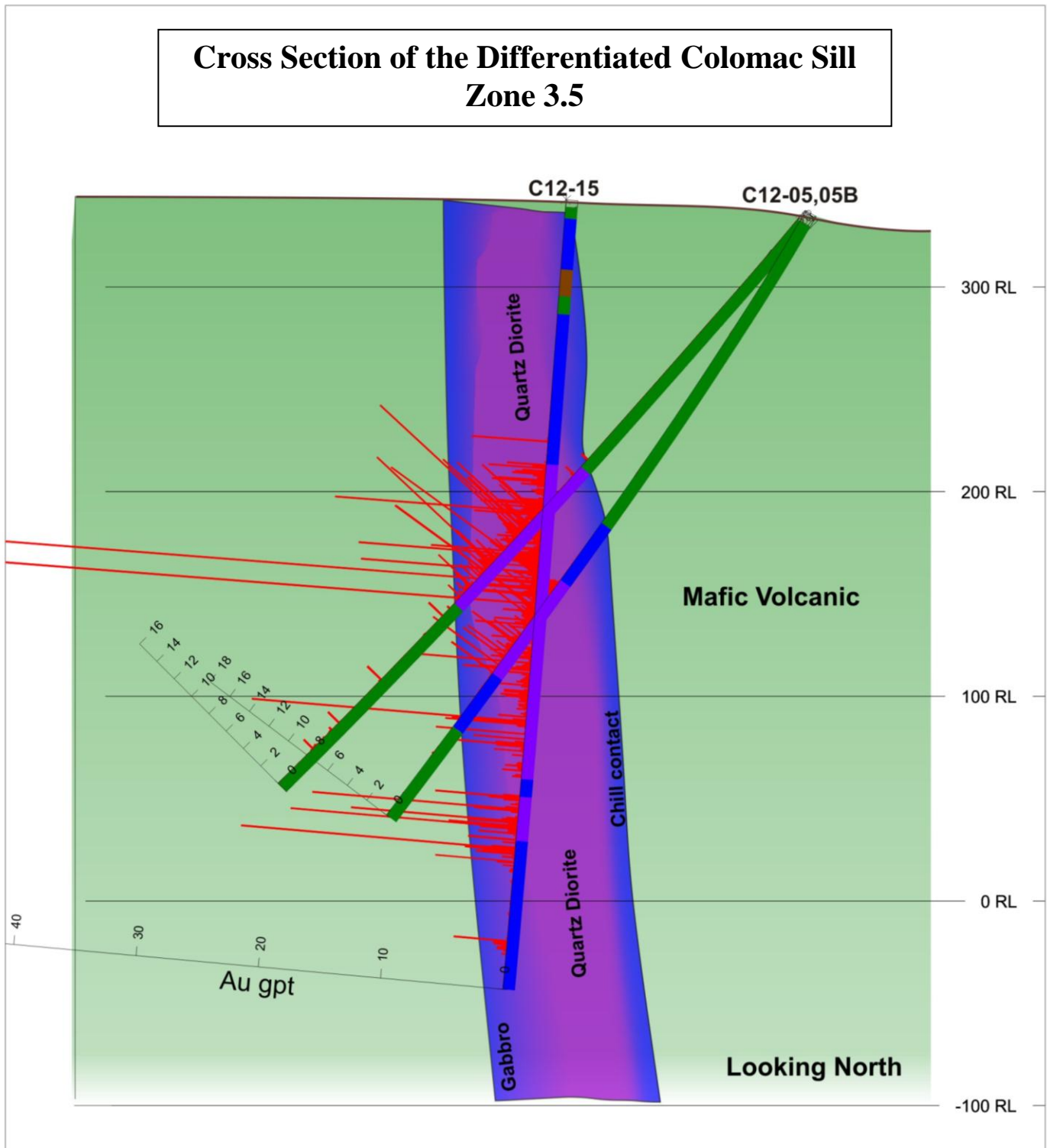
Figure 1. C12-15 and C12-5,5B Cross Section
