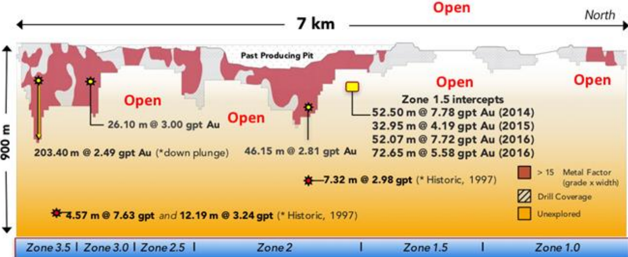
Figure 2. Colomac Longitudinal Section Showing Near Surface Resource and Exploration Potential
