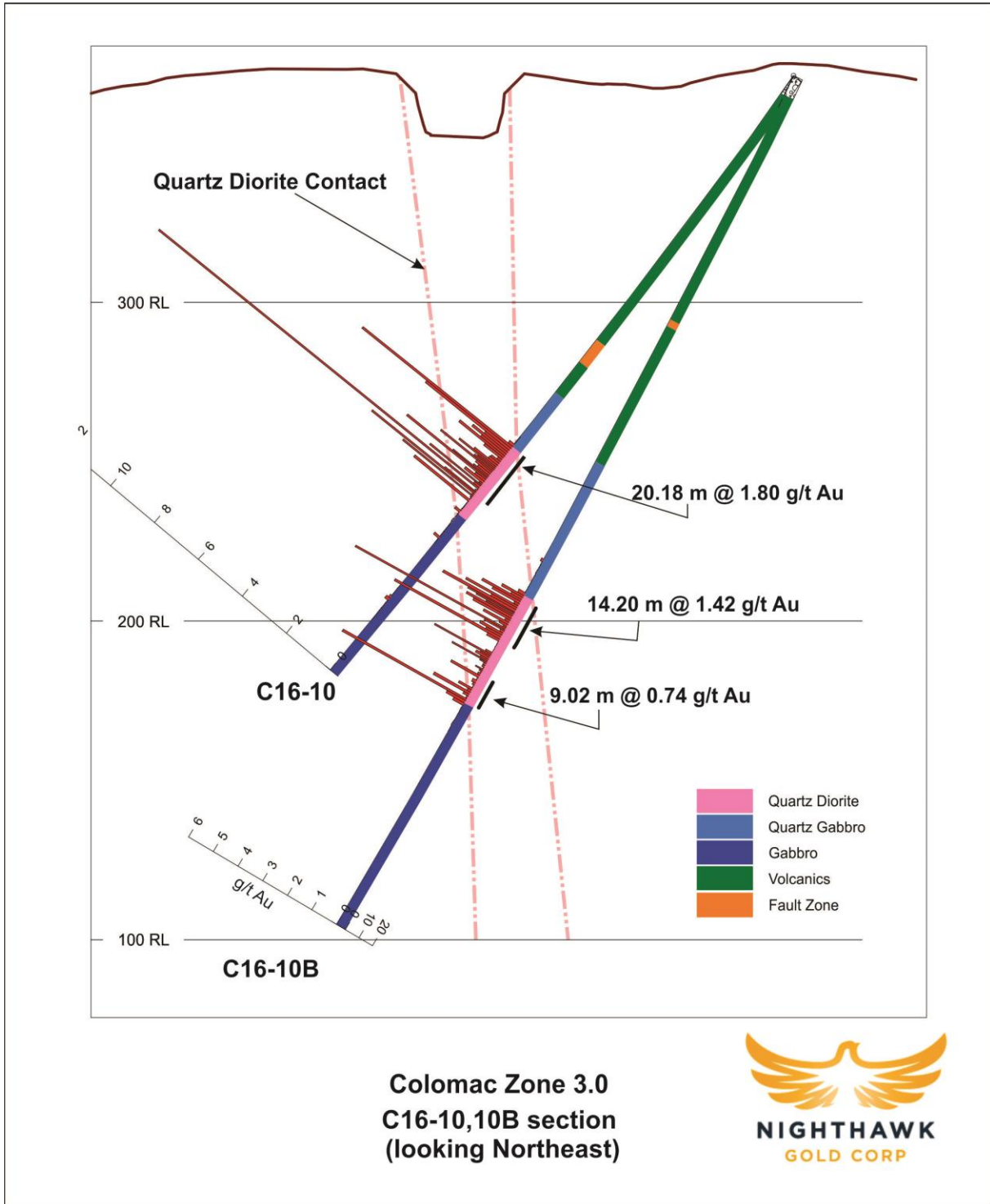
Figure 3. C16-10, -10B Drillhole Section
