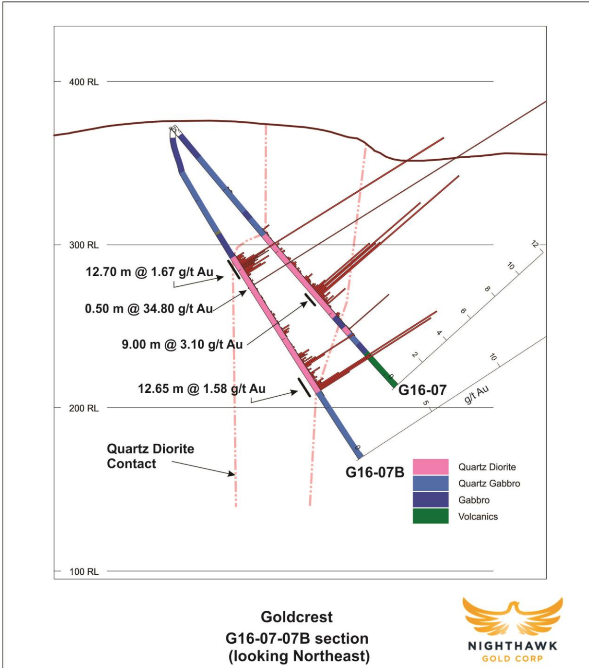
Figure 4. G16-07, -07B Drillhole Section
