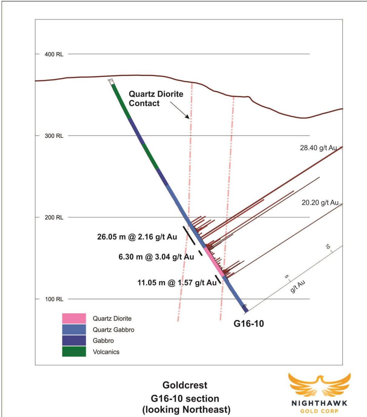
Figure 5. G16-10 Drillhole Section
