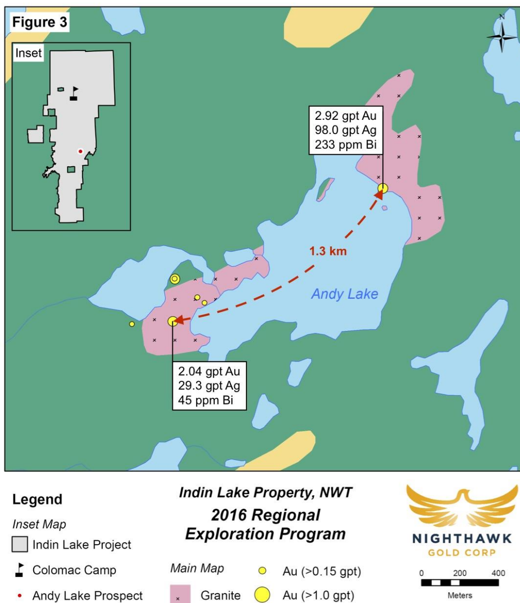
Figure 3: Map of the Andy Lake area showing high Au-Ag-Bi mineralized sample locations.
