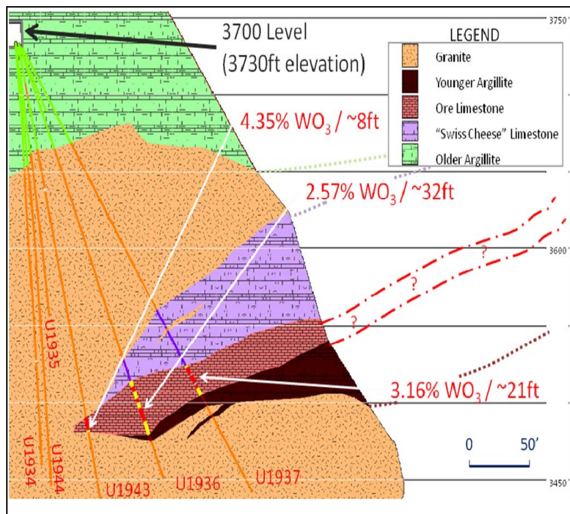
Figure 2. Non-orthogonal cross-section, looking approximately North, of new diamond drill holes. Holes U1944, U1934 and U1935 (leftside ) all ended in granite.
