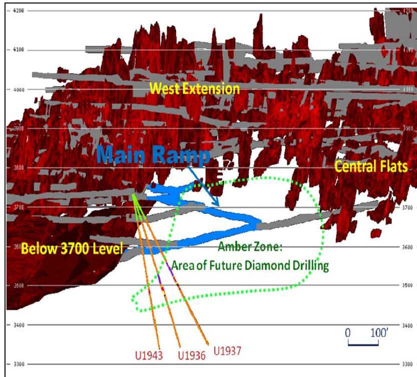
Figure 1. Long section, looking approximately North, showing the location of reported diamond drillholes relative to 3D model of existing workings and known orebodies (in red).
