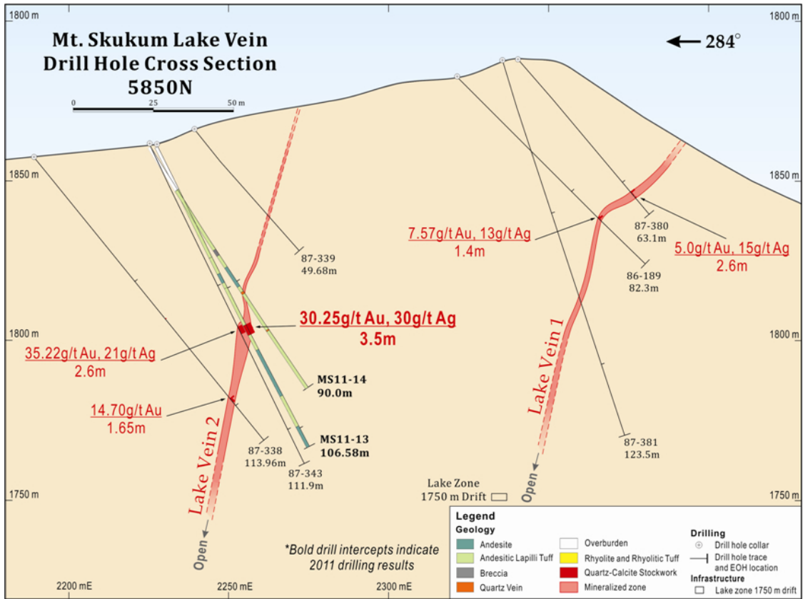
Schematic 3 – Additional Section of Mt. Skukum Lake Zone Geologic interpretations
