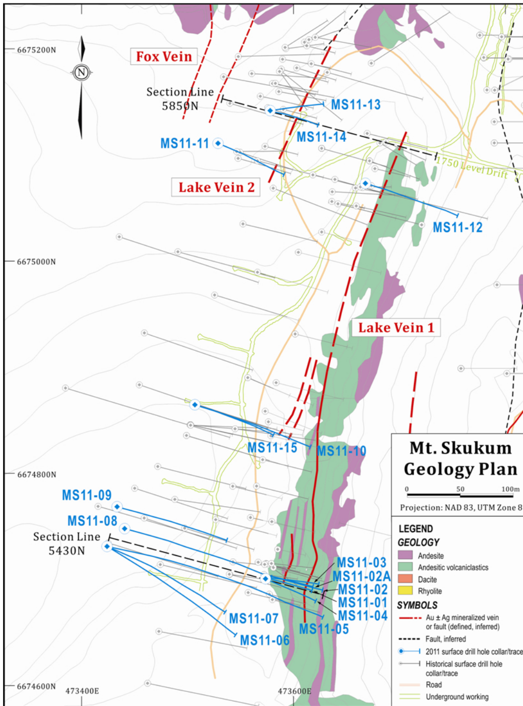
Schematic 1 – Overview of Mt. Skukum Lake Zone Geology
