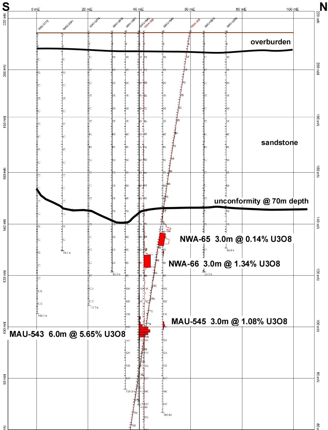
Figure 2: Zone A Cross Section. Grid is 20x20m, uranium intercepts are in red.
