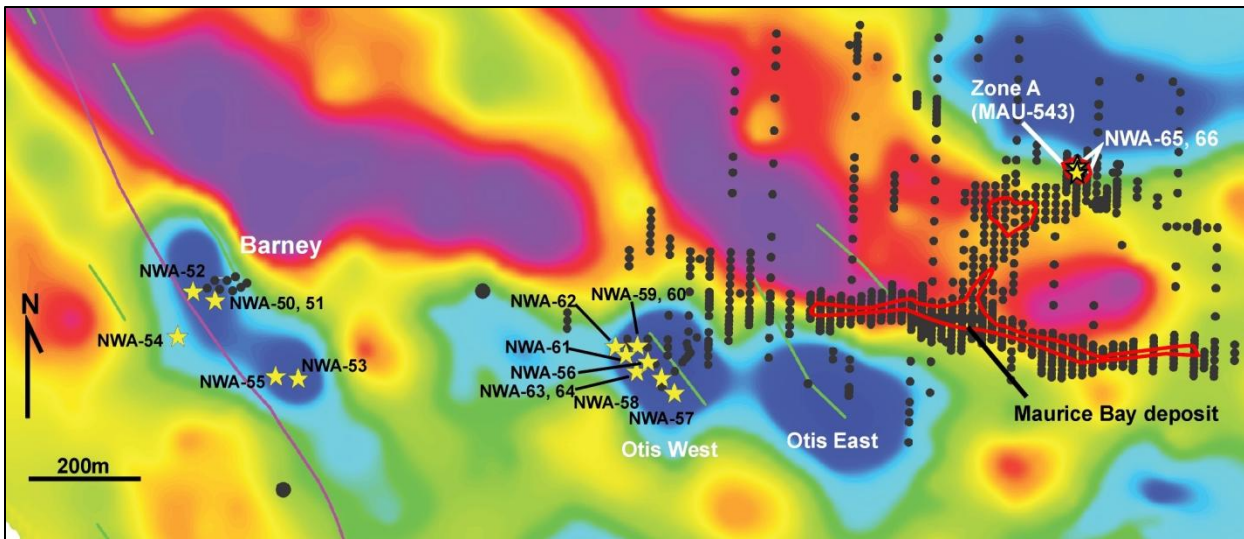
Figure 1: Gravity with Drill Targets on the NW Athabasca Project. Black dots are previous holes, yellow stars are holes drilled in 2013 by Forum. Lines are EM conductors. Gravity lows are depicted as blue colours.
