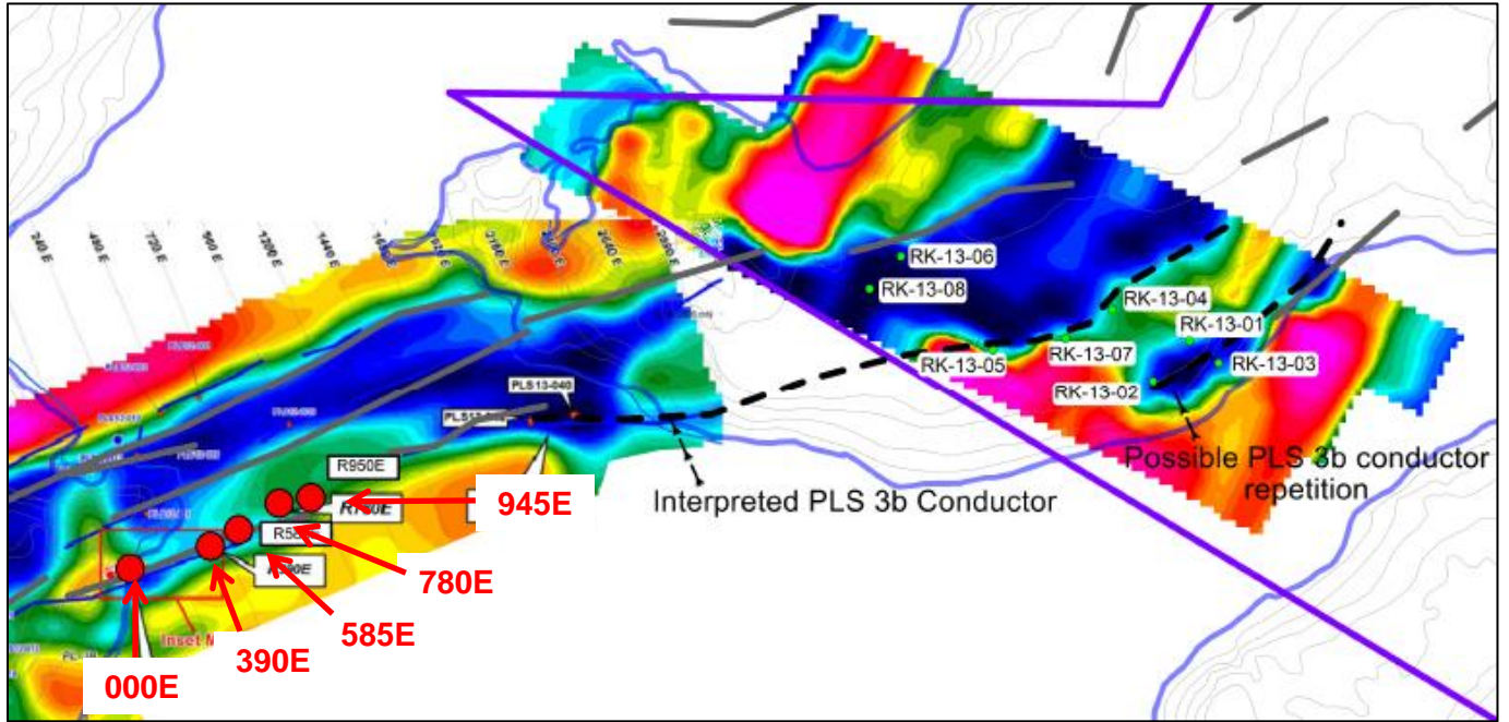
Fig 1 NexGen Rook 1 drill hole locations on DC resistivity image
