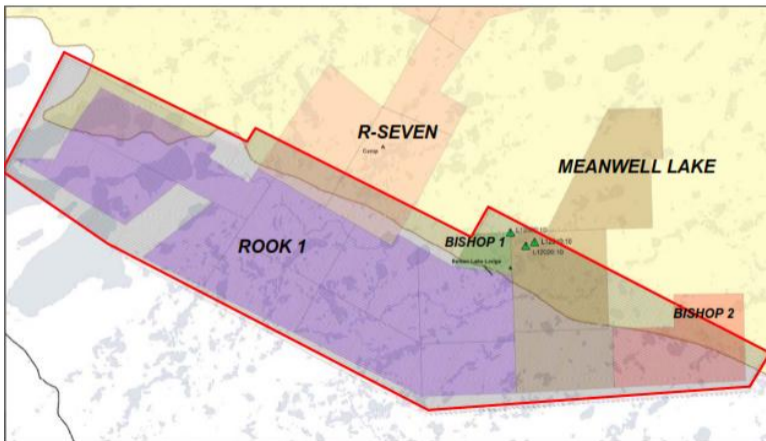
Figure 2 Planned radiometrics / magnetics / EM survey over Rook I and adjoining South-West Athabasca Basin Margin properties
