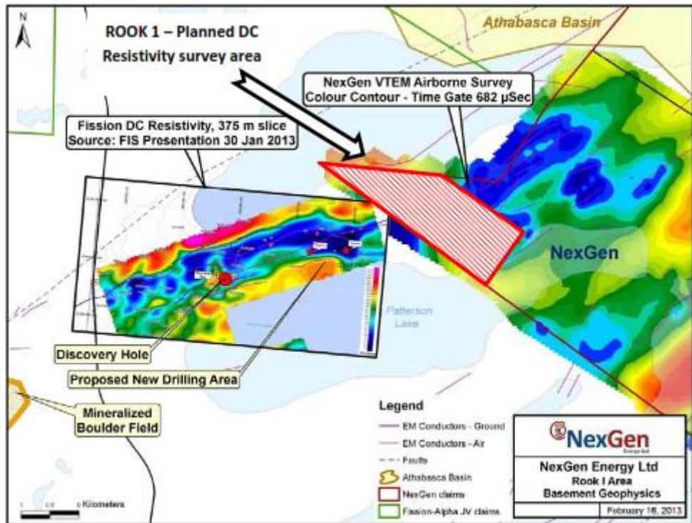
Figure 1 – Rook I, Planned resistivity grid
