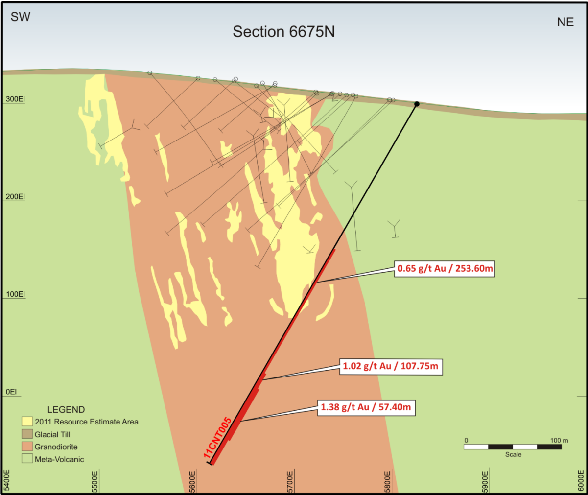
Figure 1 - Cross Section 6675N
