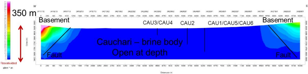
Figure 3: Cauchari North AMT line with Orocobre drill holes projected onto the section
