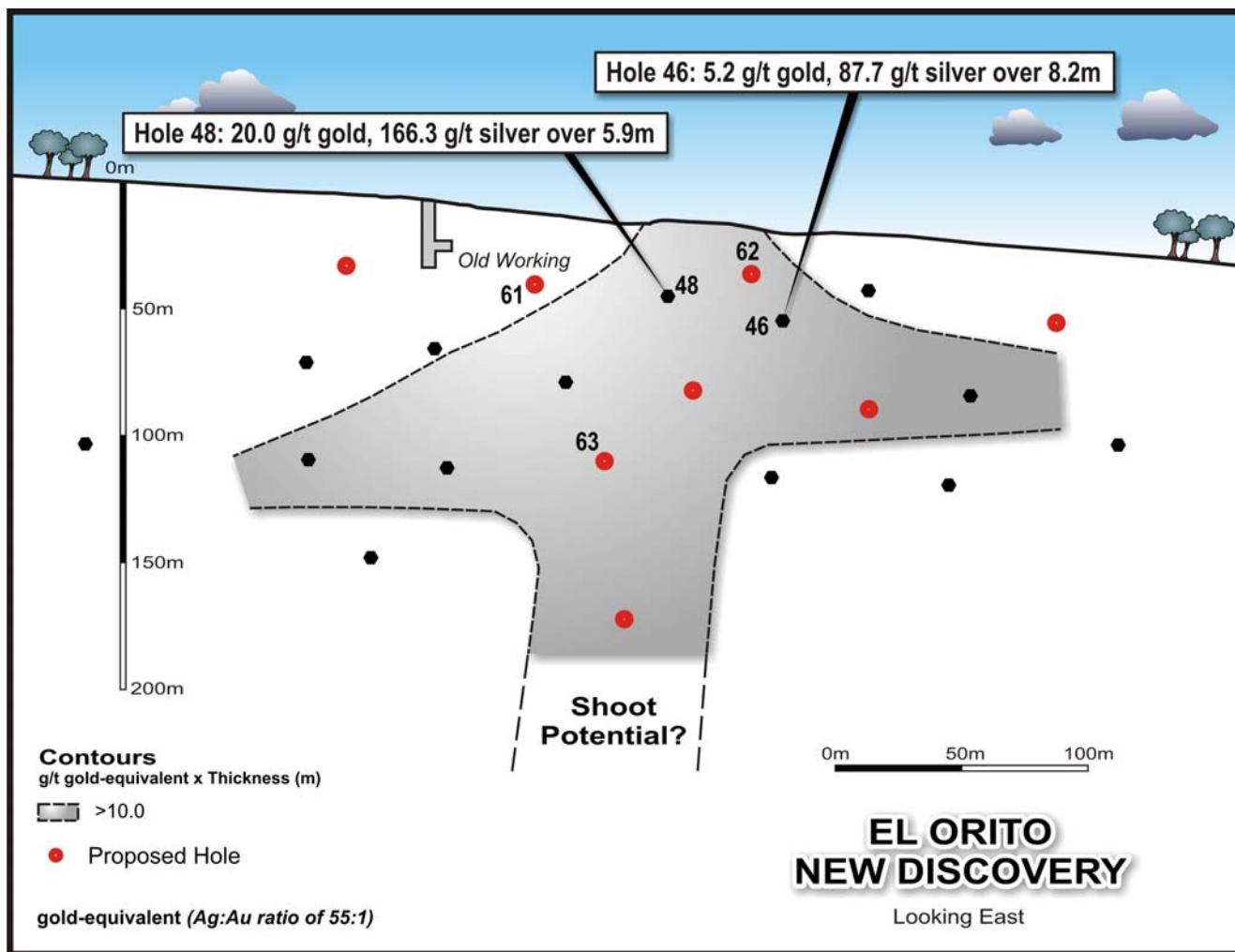
Figure 2 – El Orito Long Section
