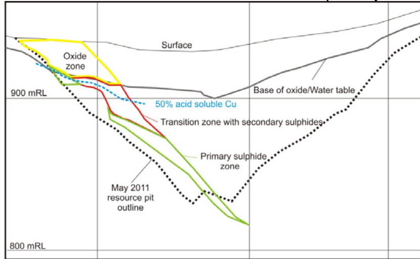
Figure 2. Principal relationships between the oxide, transition and primary sulphide zones in the Central lode of the Karchiga deposit. Dashed blue line shows schematic position of the dividing line between heap leachable and floatable sulphides from the transition zone. The area above the 50% acid soluble Cu line is potentially amenable to heap leaching.
