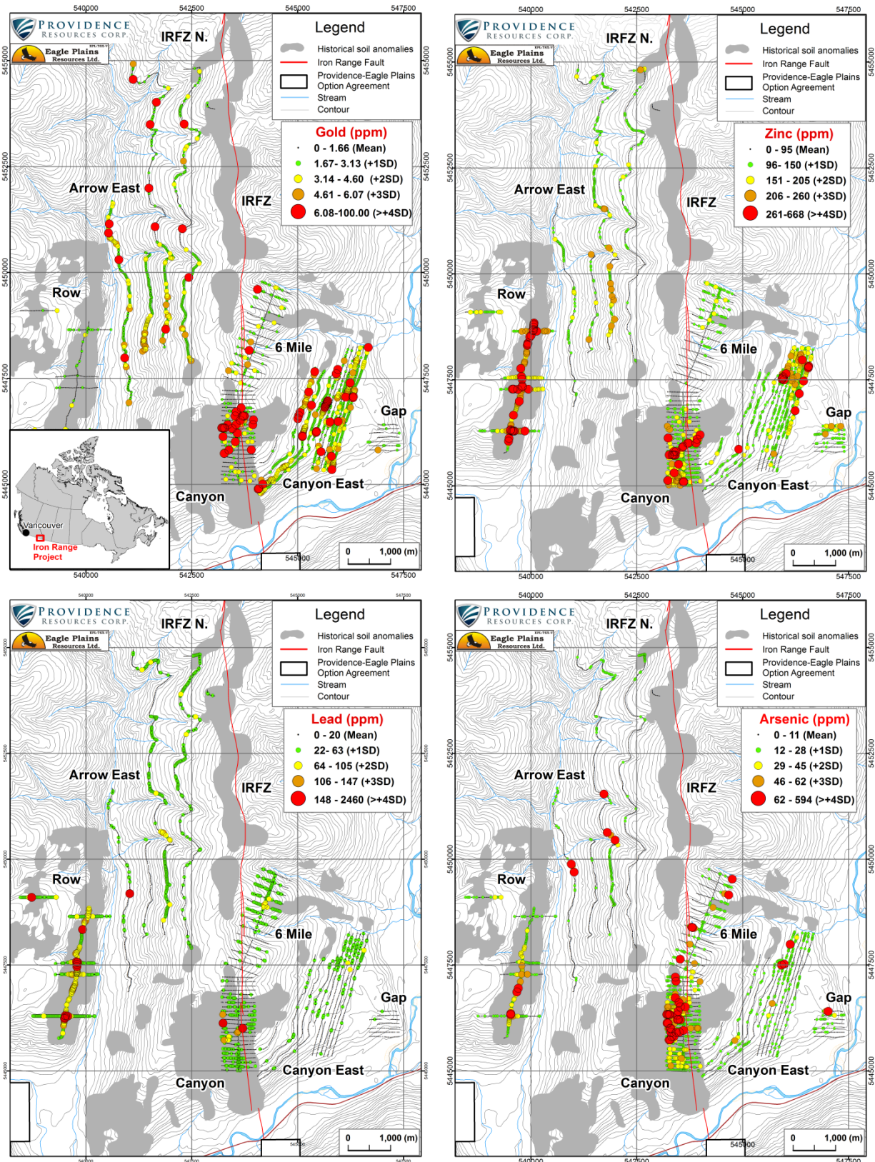
Figure 1. Providence Resources 2011 soil gold (Fig. 1A), zinc (Fig. 1B), lead (Fig. 1C), and arsenic (Fig. 1D) geochemistry results. Sample location bubble plots are scaled in size and are colour coded to show anomalous samples in order of increasing standard deviation above the mean value.
