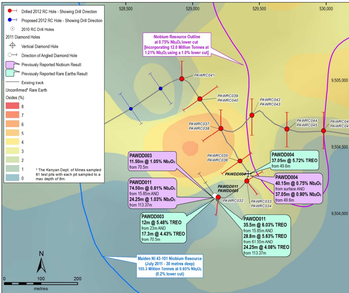
Figure 2: Location of currently drilled 2012 RC holes (results pending) and historic PAW diamond holes with TREO and Niobium grades (Insert shown in figure 1).
