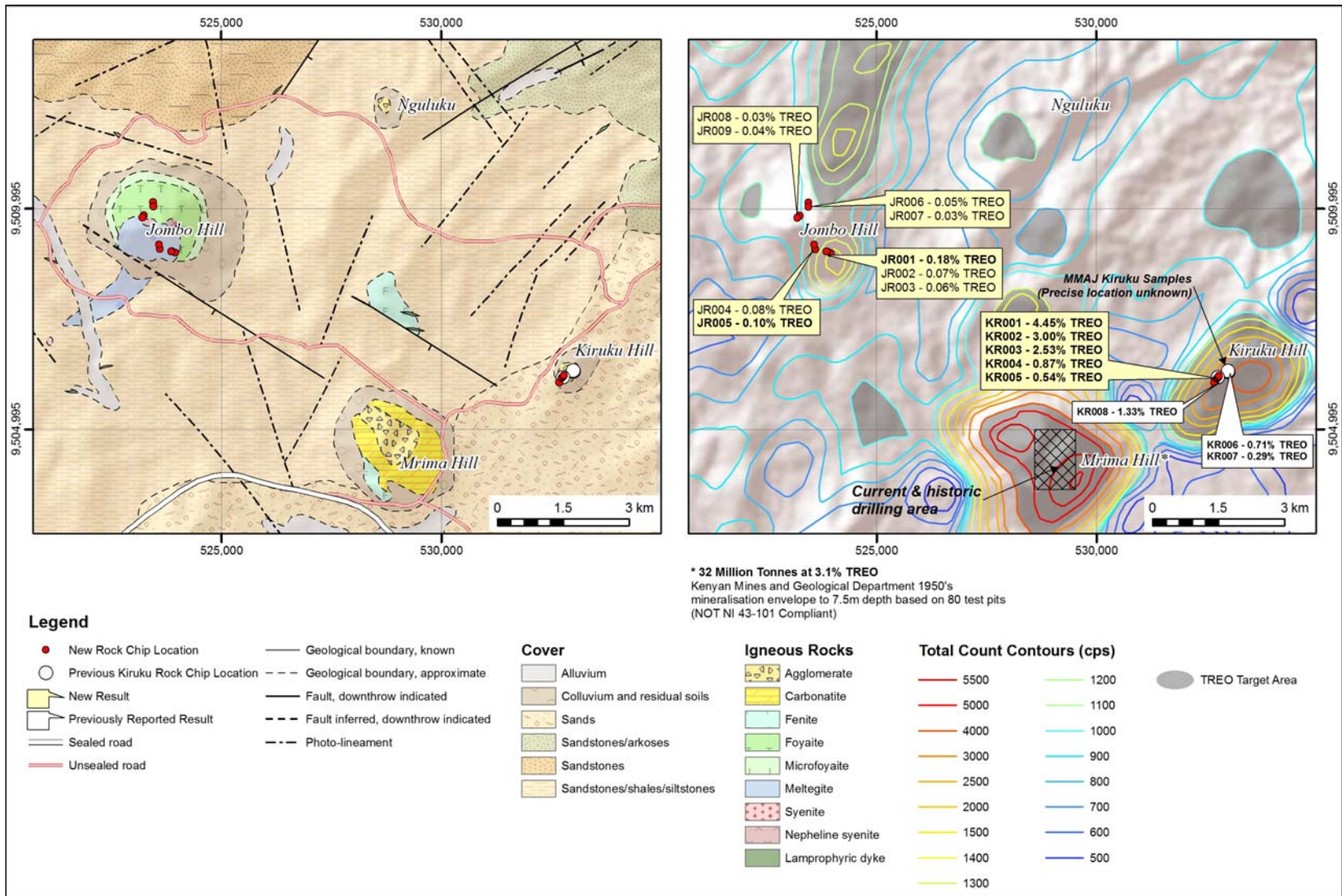
Figure 1: Left: Geology of the Mrima Hill area sourced from MMAJ (1993). Right: Total Count radiometric data over the Mrima Hill region sourced from the Terra Surveys Limited (1977) of Canada aerial Total Count Contour plan.
