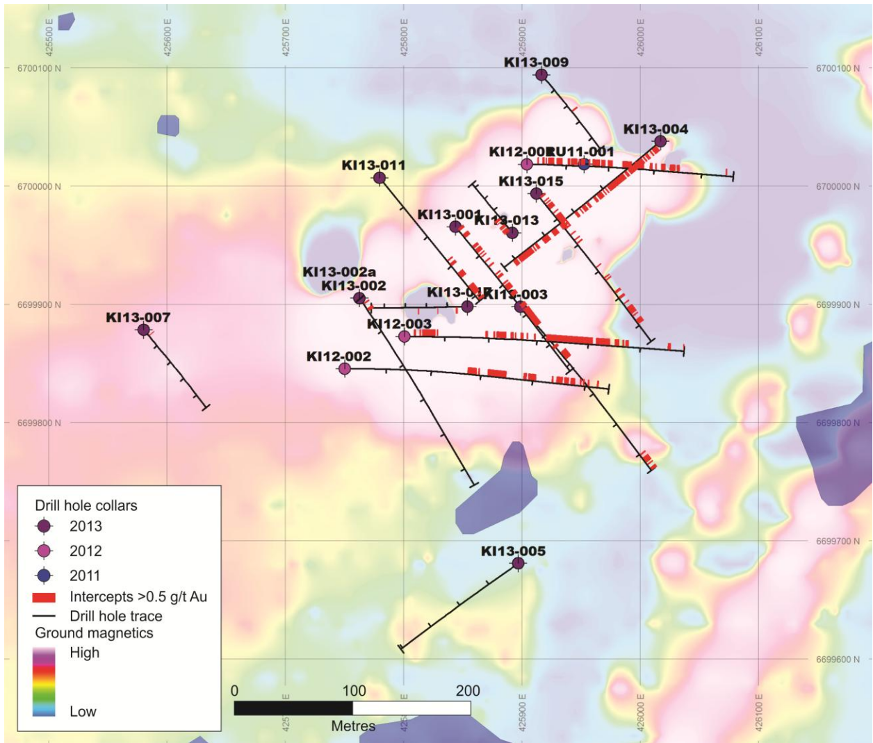
Figure 1. Rusty Drill Plan (shows all +0.5 g/t Au intercepts)
