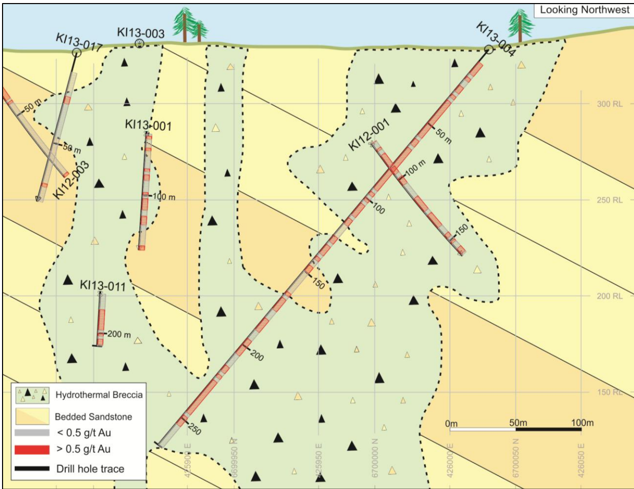
Figure 3. Rusty cross section (with geology)
