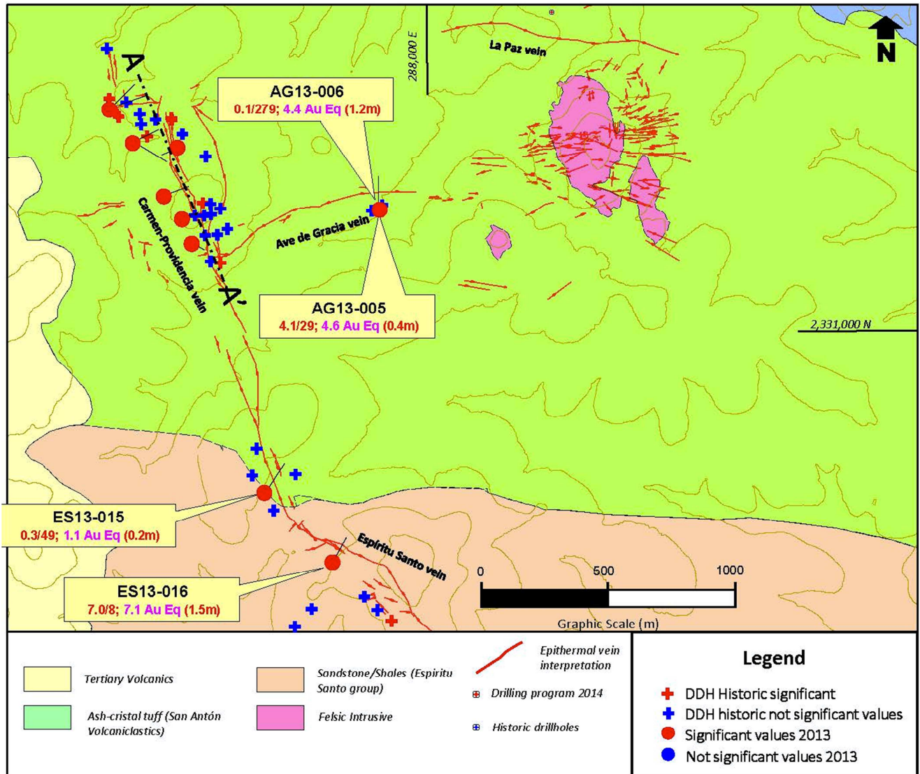
Figure 1: Cerro del Gallo Drill Hole Location Plan View
