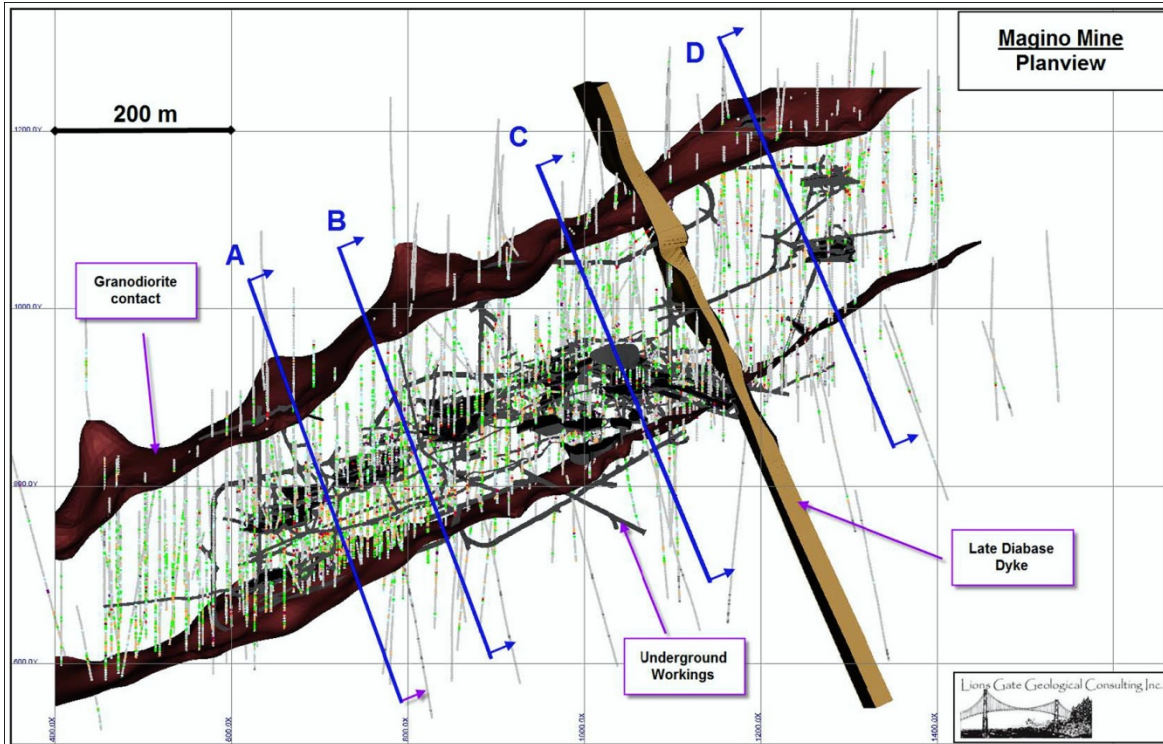
Three dimensional geologic model showing diamond drill holes, historic underground workings, contacts of the Webb Lake granodiorite stock and the principal post-mineral diabase dyke.
