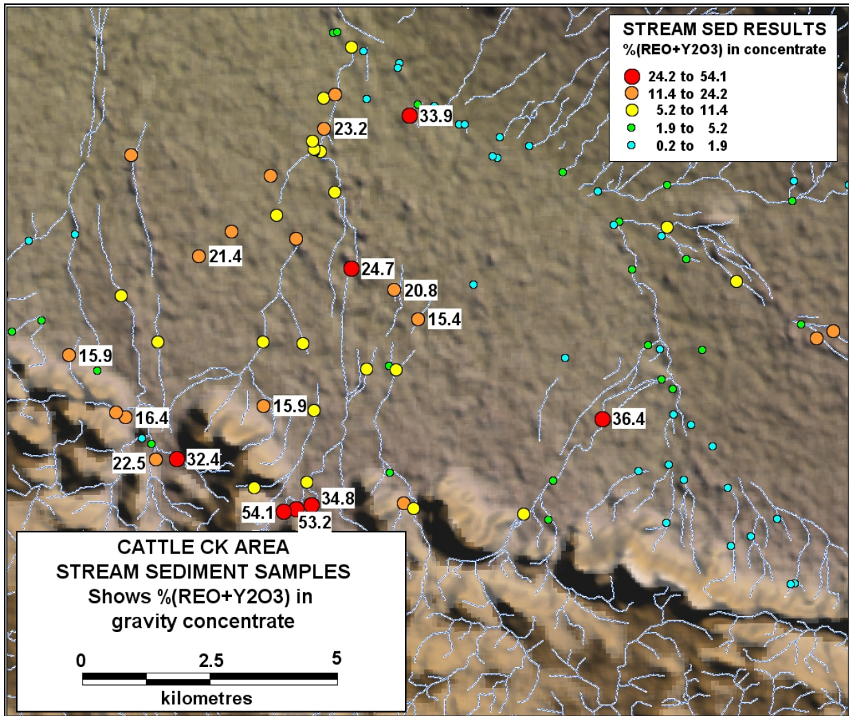
Figure 3 – Shows locations of stream sediment samples for Cattle Ck area with anomalous Total Rare Earth Oxides plus Yttrium Oxide (TREO+Y 2 O 3 ) in heavy mineral concentrate highlighted
