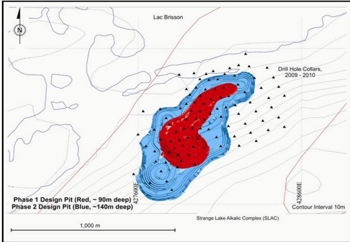
Figure 4: Phase 1 and Phase 2 Pit Design
