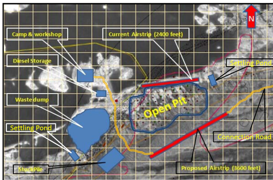
Figure 1 – Conceptual Layout of Infrastructure, Strange Lake B-Zone Open-Pit Operation
