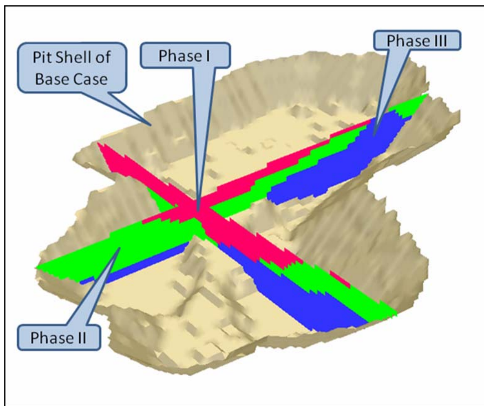
Figure 2 – Strange Lake B-Zone Deposit Open-Pit Shell Outline Model and Development Sequence
