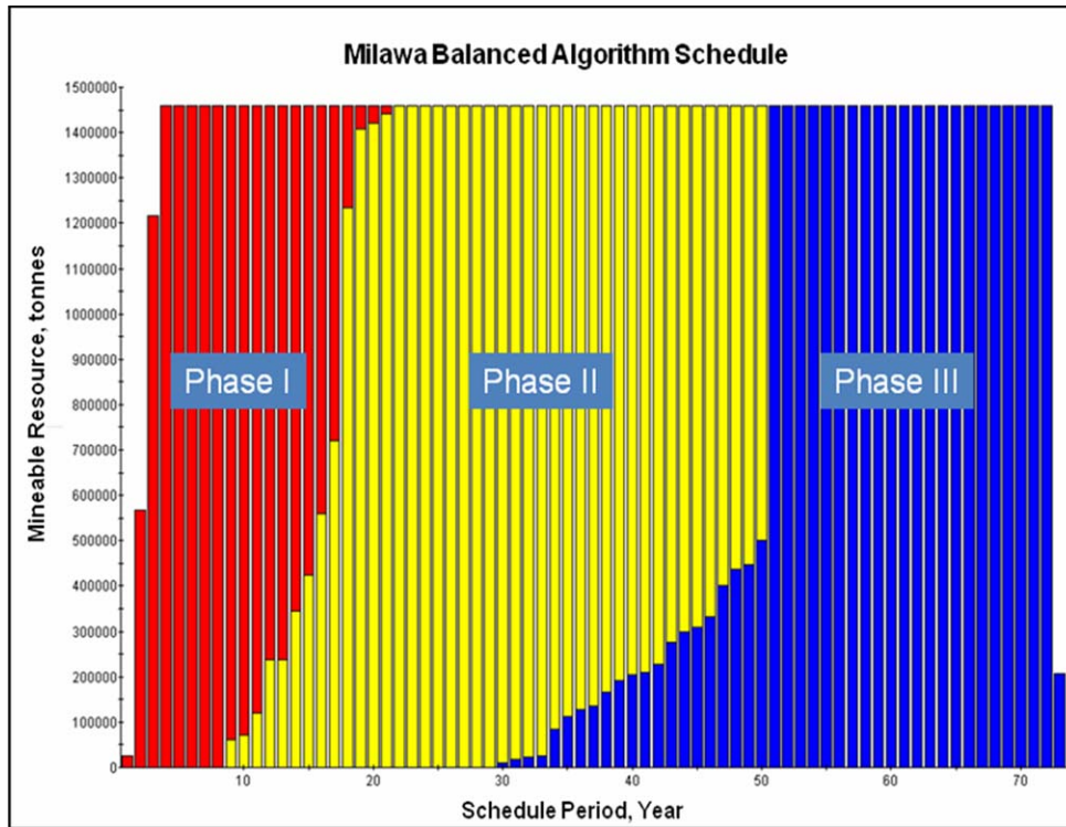
Figure 3 – Strange Lake B-Zone Life-of-Mine Production Sequencing
