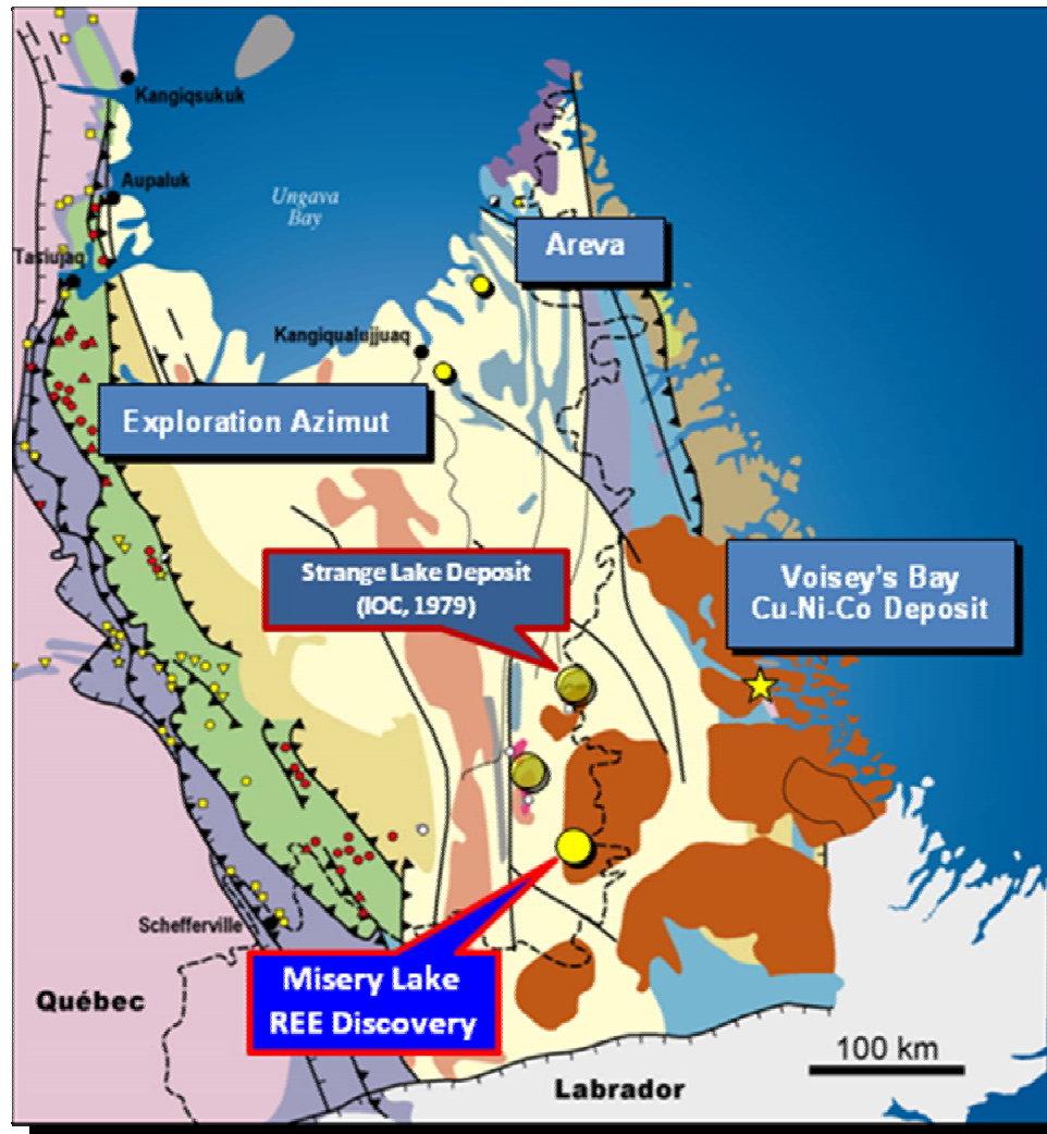
Figure 1 – Misery Lake Project Location Map, George River area, Québec
