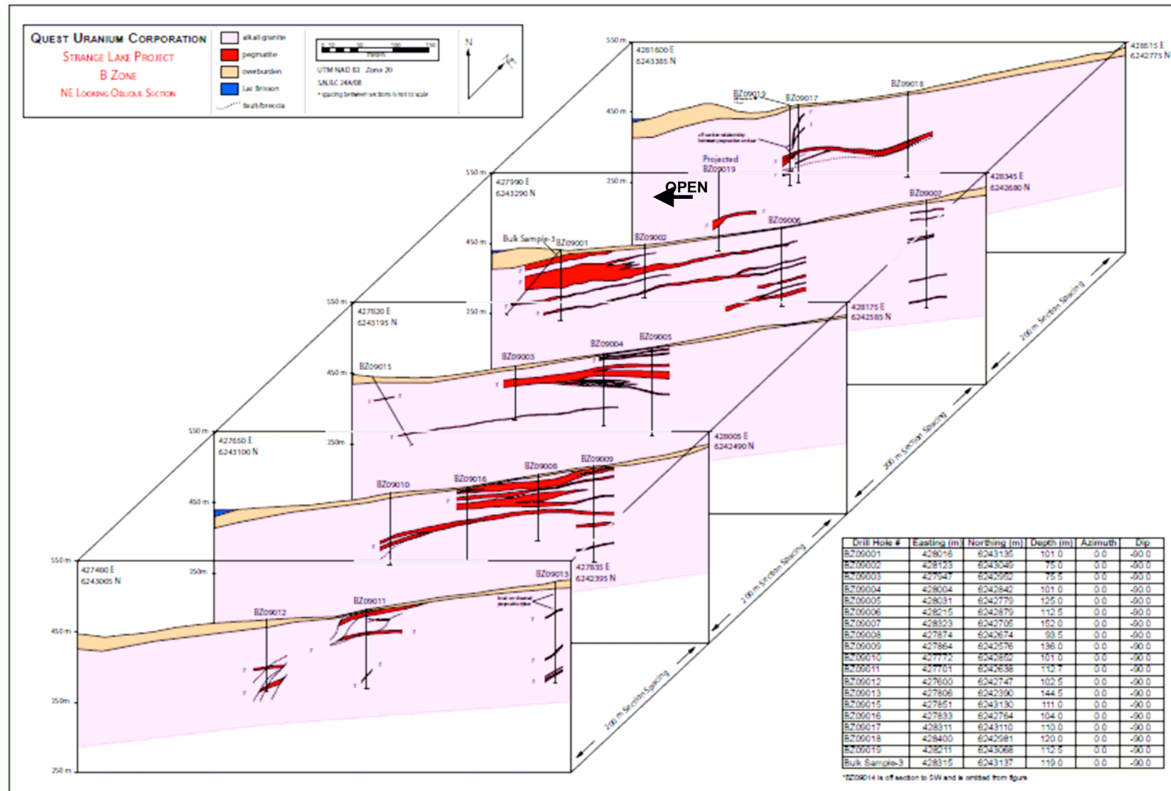
Figure 4 – B-Zone Oblique Composite Geological Cross Section, Strange Lake Project, Quebec
