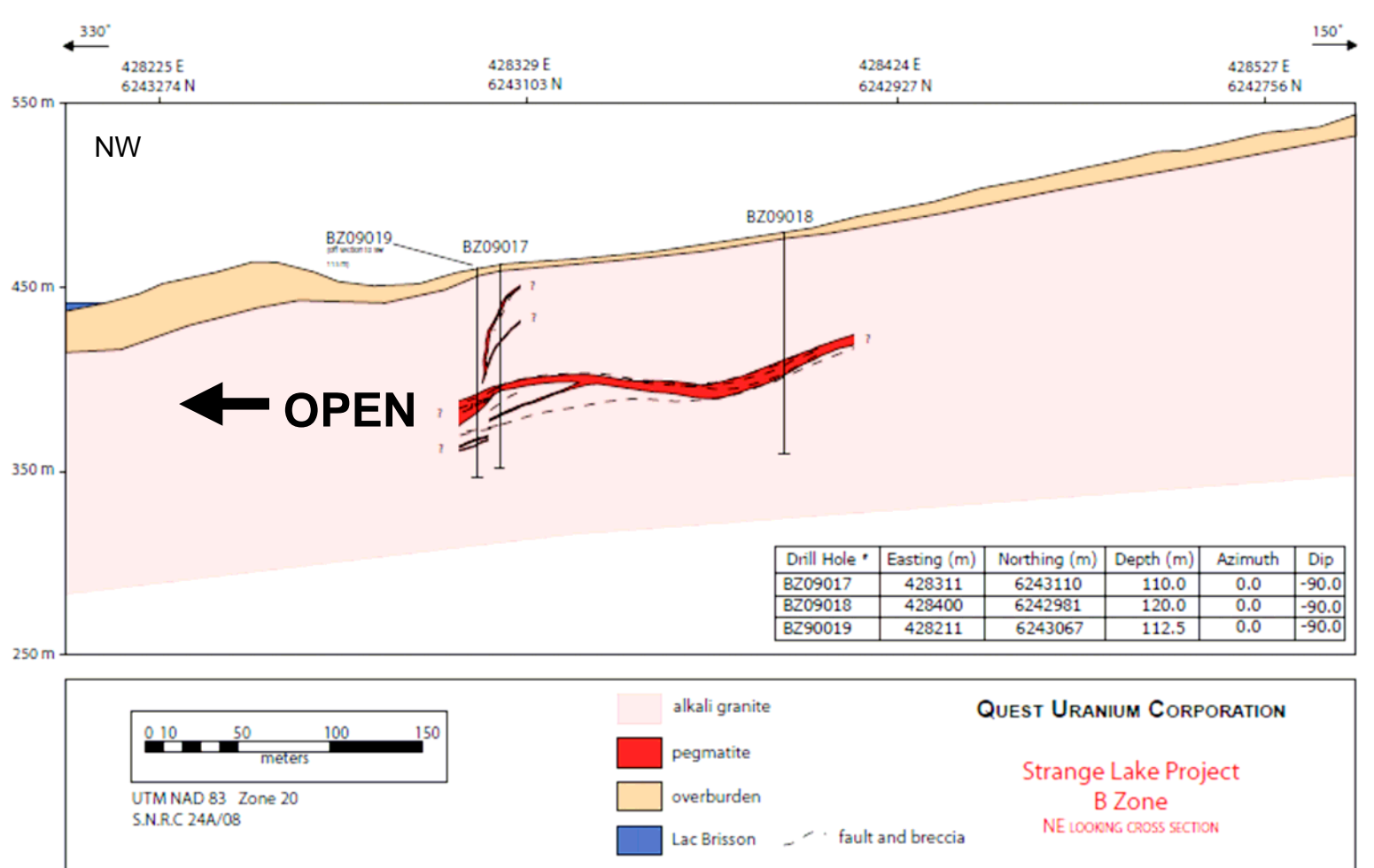
Figure 5– B-Zone Geological Cross Section 0+00, Strange Lake Project, Quebec
