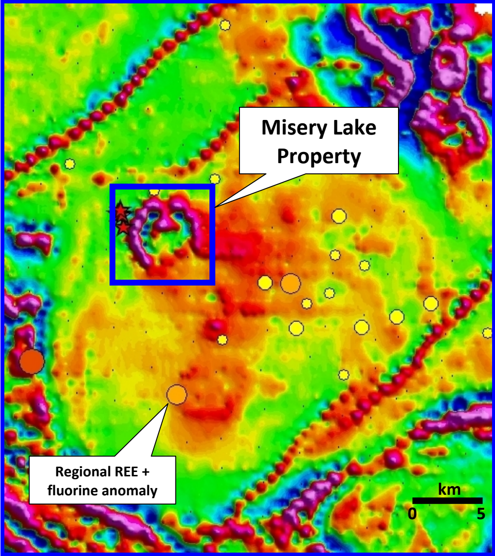
Figure 2 – Misery Lake REE Discovery represented on Regional Airborne Magnetics Map, George River area, Québec
