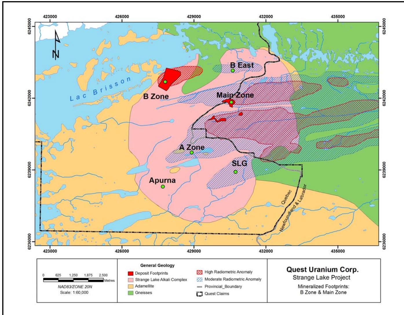
Figure 2 – Geology and Mineralization Compilation Map, Strange Lake Project, Québec
