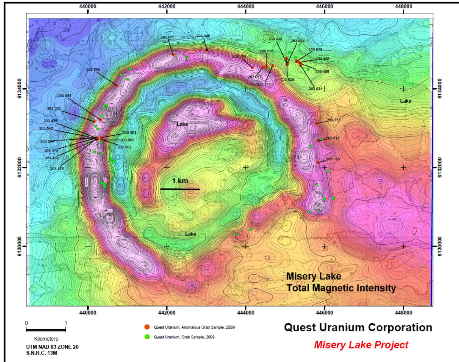
Figure 3 – Misery Lake Discovery Grab Sample Location Map on Airborne Magnetics, Québec
