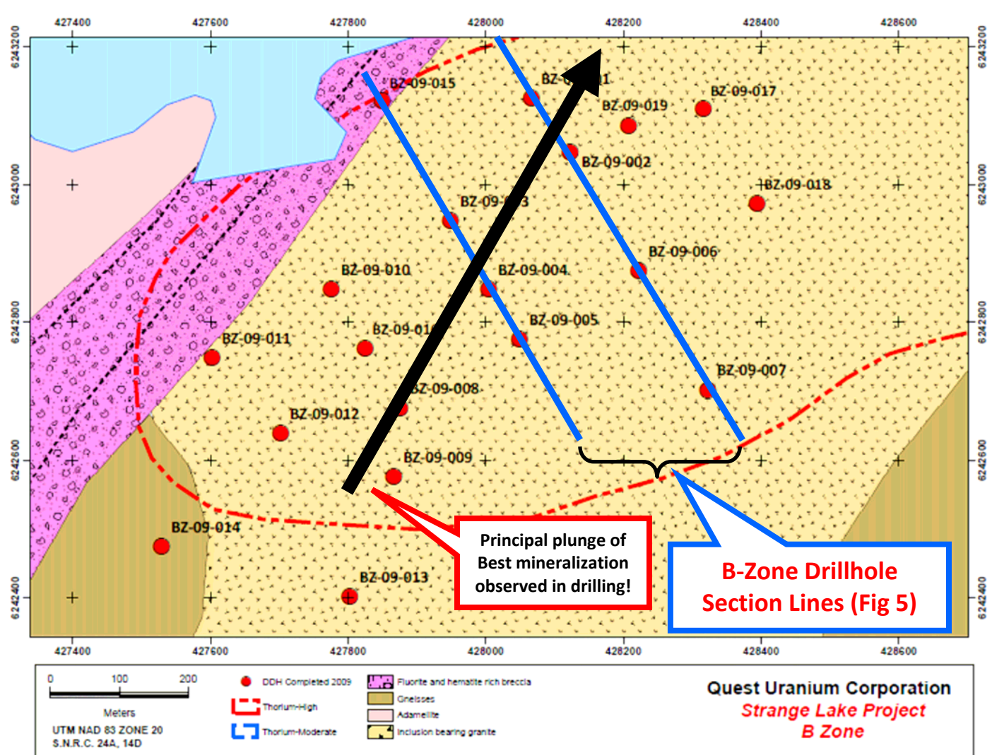
Figure 3 – B-Zone Drillhole Location Map, Strange Lake Project, Québec
