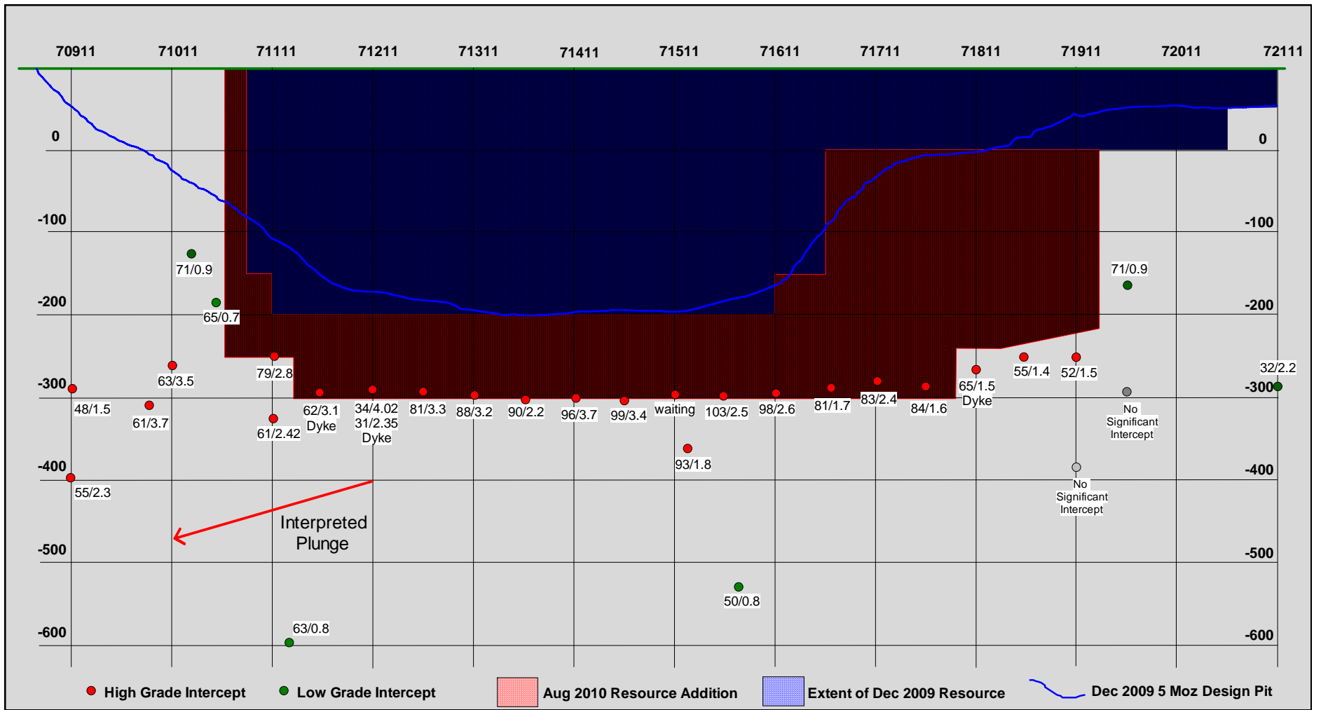
Long Section of Greenschist Zone looking West showing extent of Updated resource and intercepts of deepest hole on section
