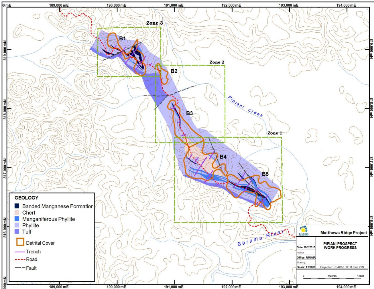
Figure 1 – Map of Pipiani Prospect showing results of exploration work done
