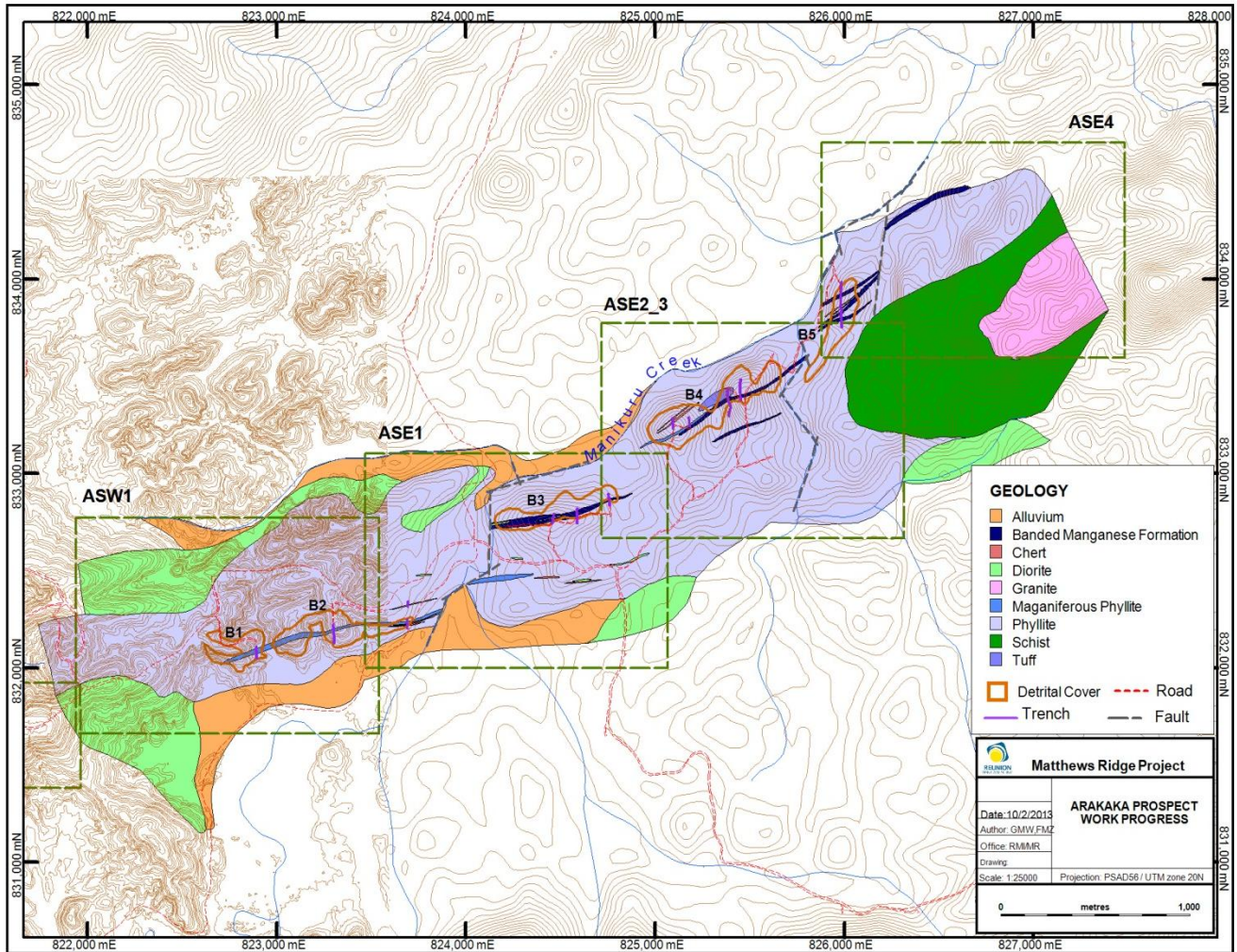
Figure 2 – Map of Arakaka Prospect showing results of exploration work done
