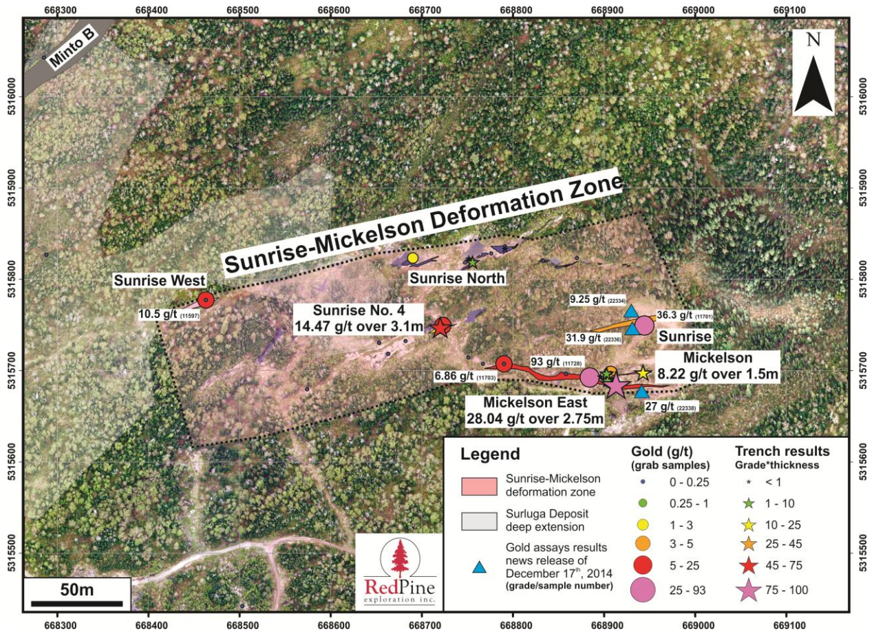
Figure 1. Gold showings of the Sunrise-Mickelson Deformation Zone
